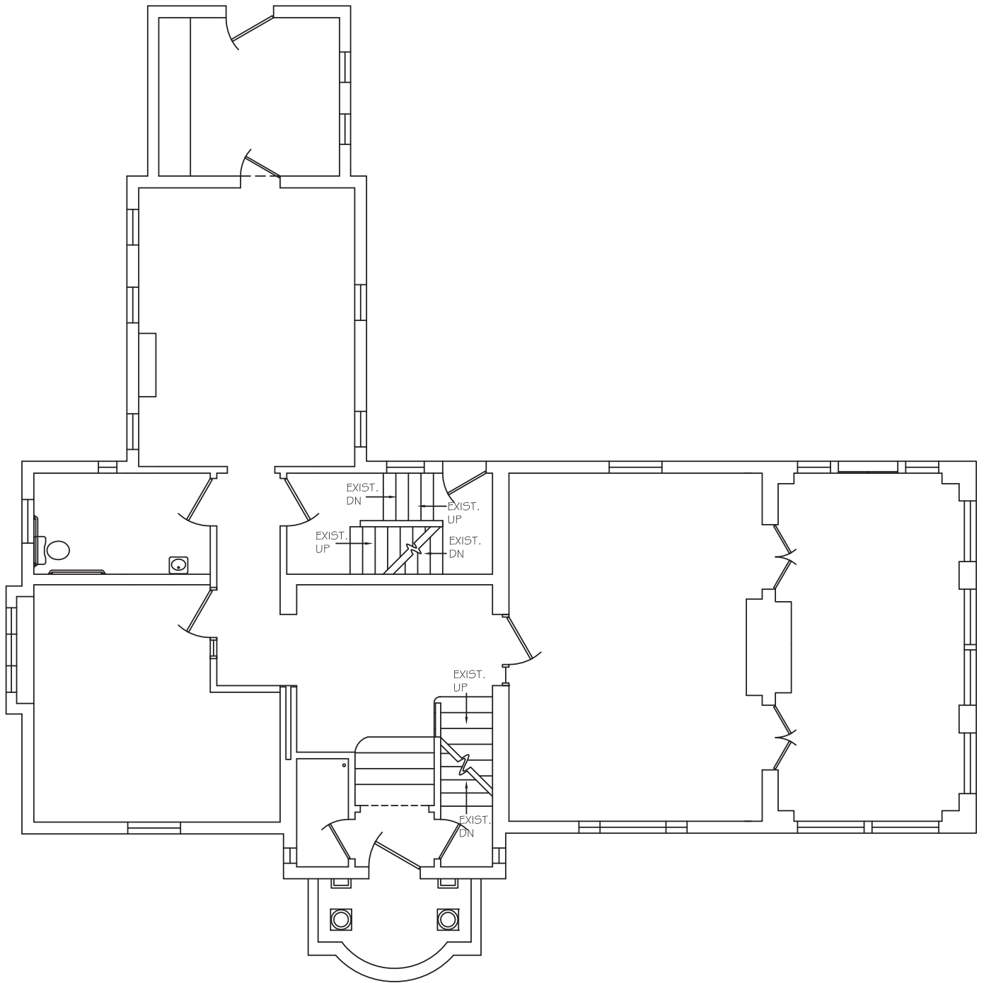
FIRST FLOOR
